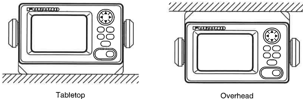
Figure 6-1 Tabletop and overhead mounting methods
