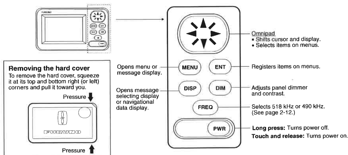
Figure 2-1 Control panel
