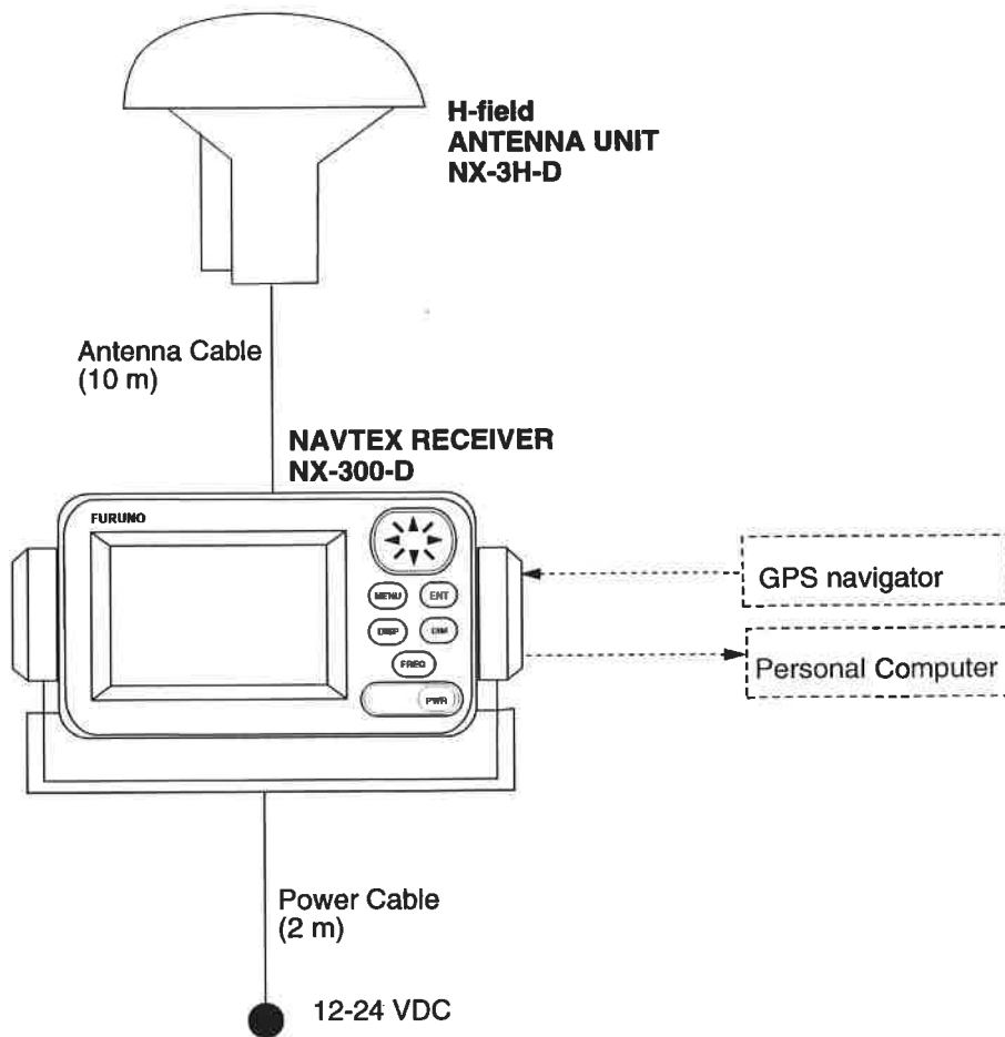
NX-300 System configuration
