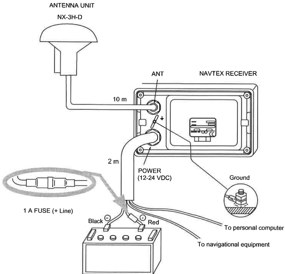
Figure 6-3 Wiring
