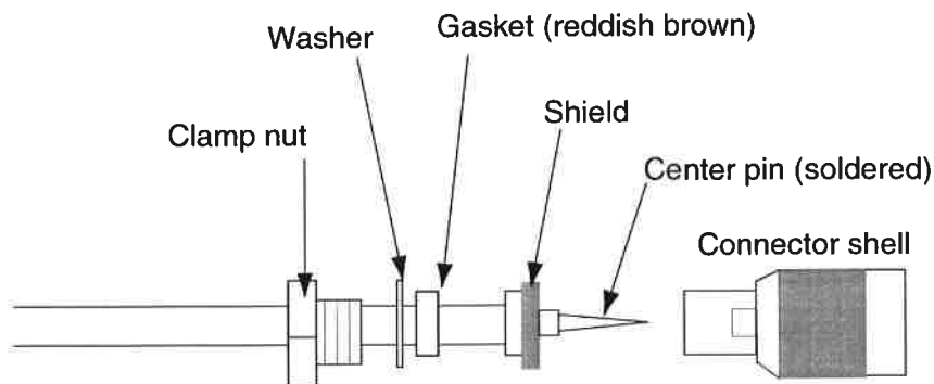
Figure 6-2 How to assemble the connector
